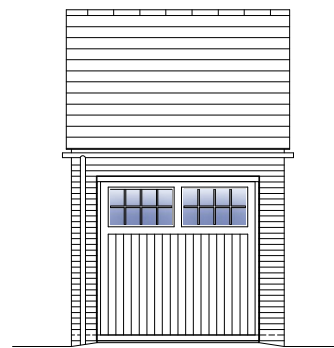
G1 FRONT ELEVATION
